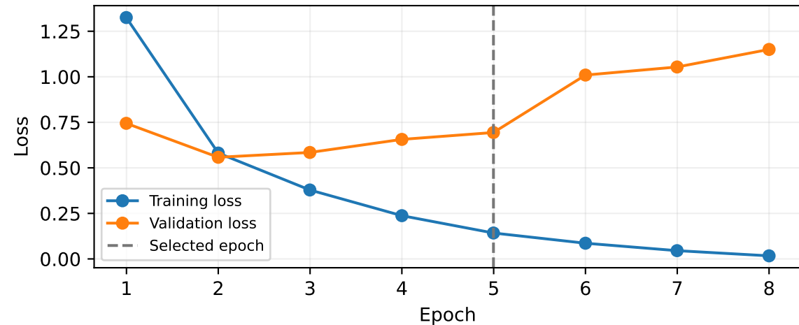
v3_600 | selected LR = 3e-05
