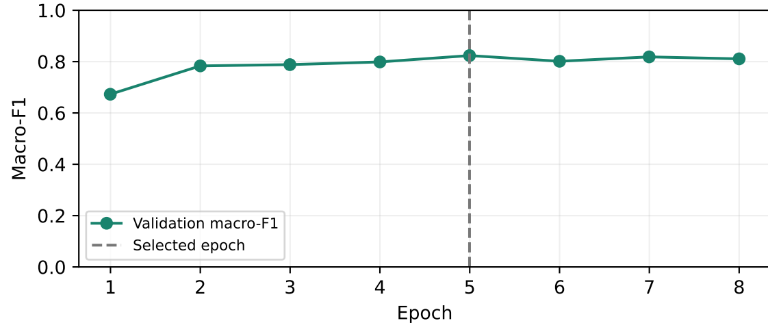
Best validation macro-F1 = 0.8236
