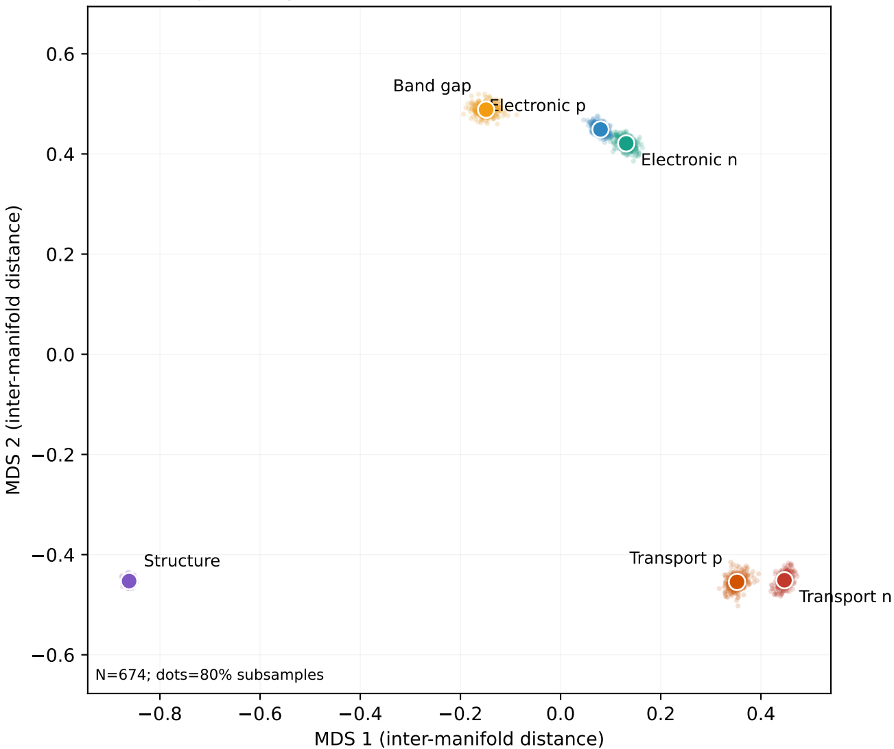
2D atlas: geometry of six feature manifolds
