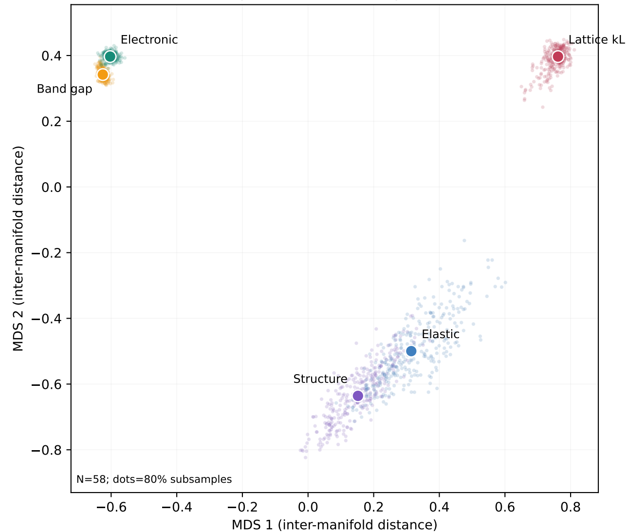
kL subset: electronic-phonon manifold separation
