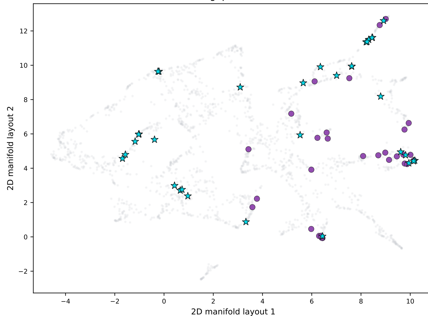
Leave-one-formula-out manifold test full-dimensional diffusion coordinates
