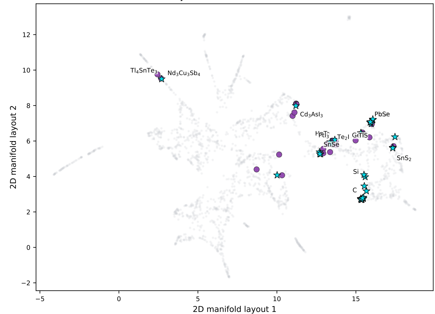
Balanced joint diffusion manifold: S1 \times E2
