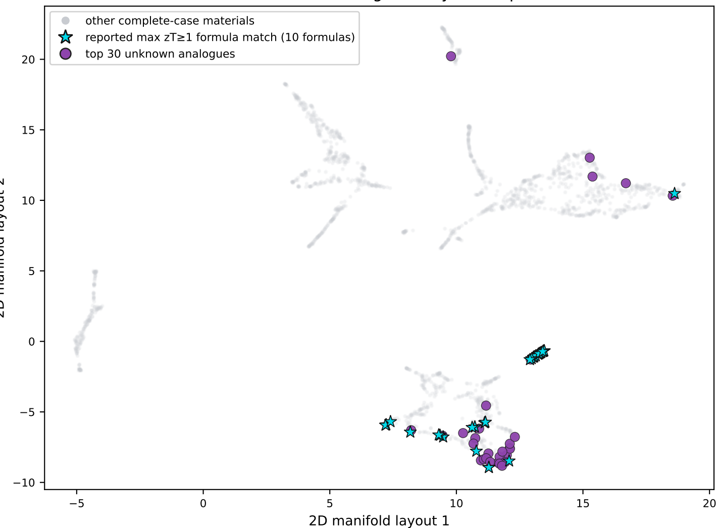
Structure manifold: S1 geometry + composition
