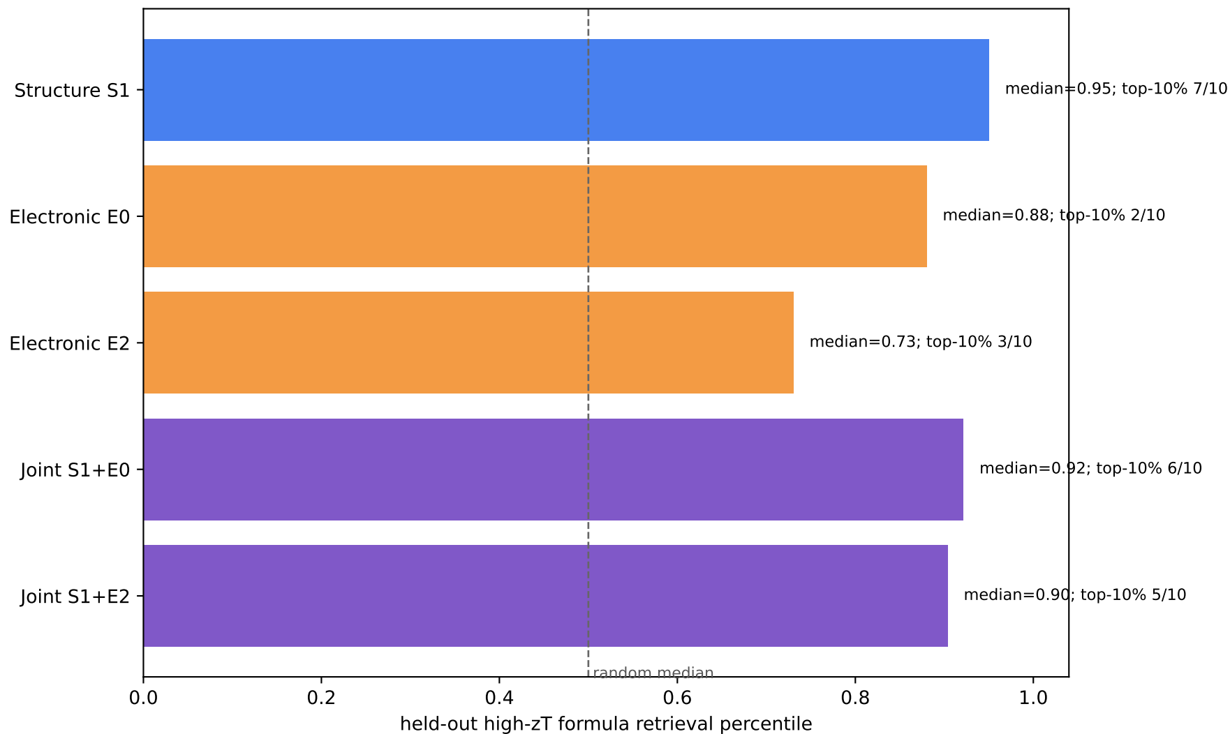
Leave-one-formula-out manifold test full-dimensional diffusion coordinates
