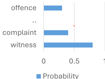
TOKEN-WISE PROBABILITY
