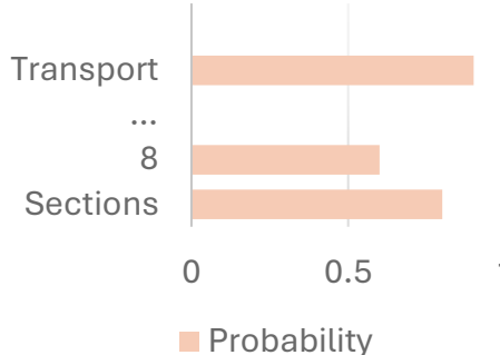
TOKEN-WISE PROBABILITY
