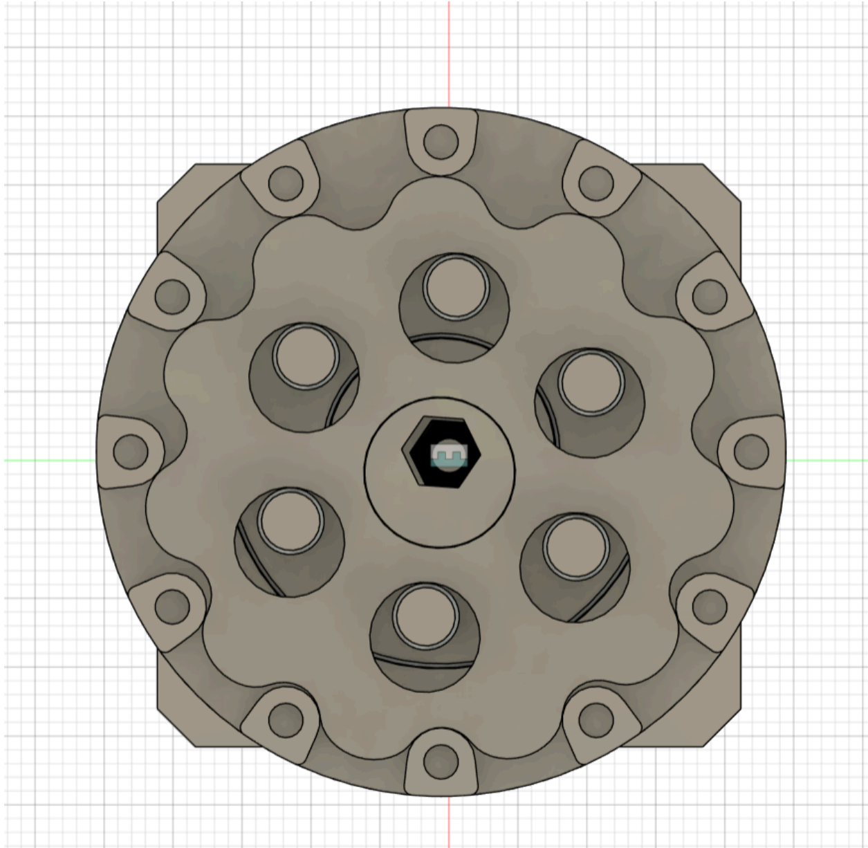
Figure 2: A top-down view of the cycloidal drive.
