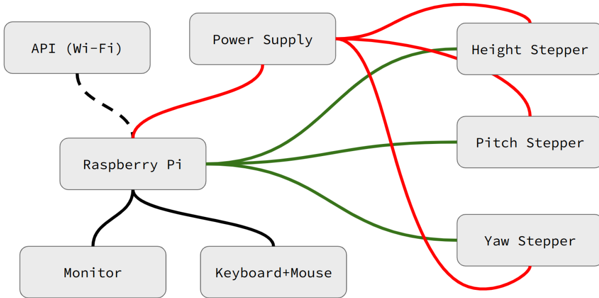
Figure 4: System physical and programmatical architecture diagram
