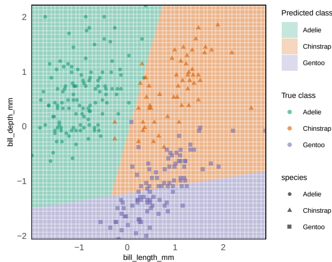
Figure 6: Decision surface of a fitted SVMODT model on the Palmer Penguins dataset.
