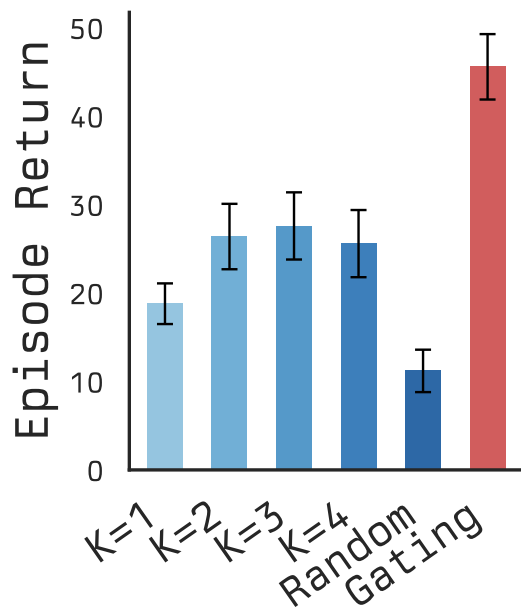
Tetris RT
