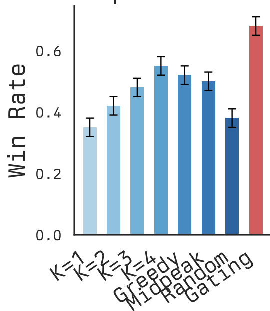
Speed Hex
