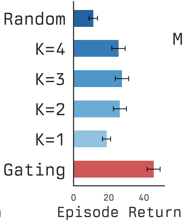
Tetris RT
