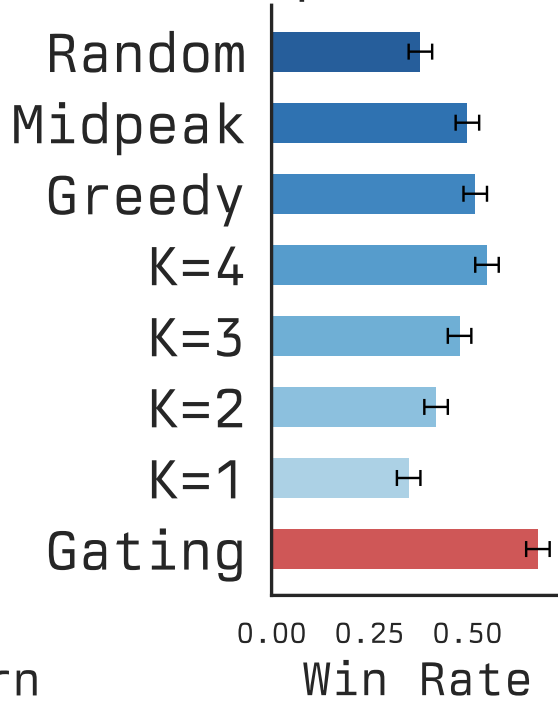
Speed Hex
