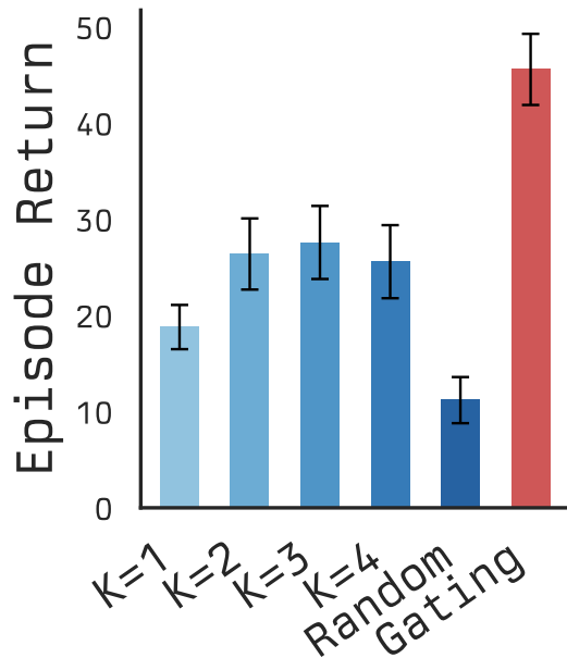
Tetris RT
