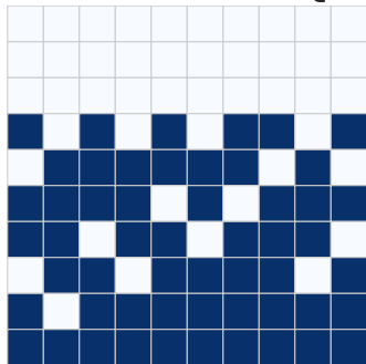
State s_t
