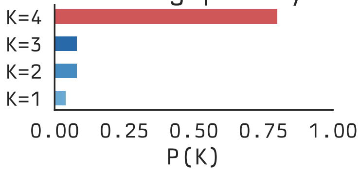
Gating policy
