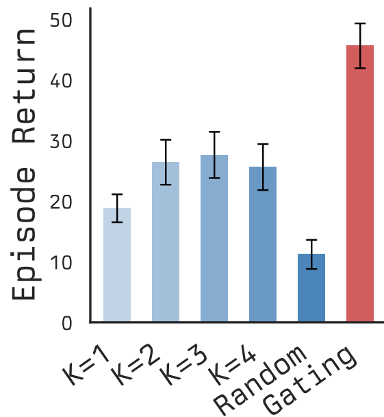
Tetris RT
