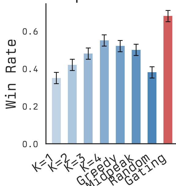
Speed Hex
