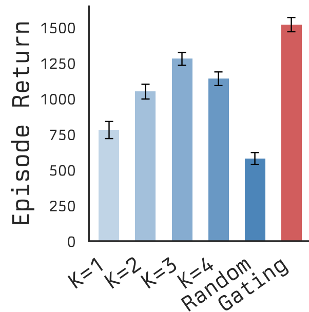
Snake
