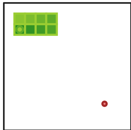
Chosen K = 2
