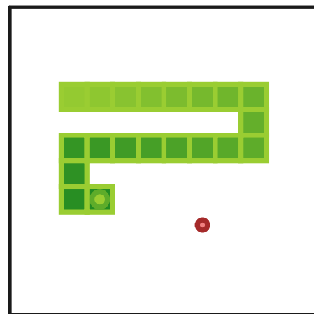
Chosen K = 3
