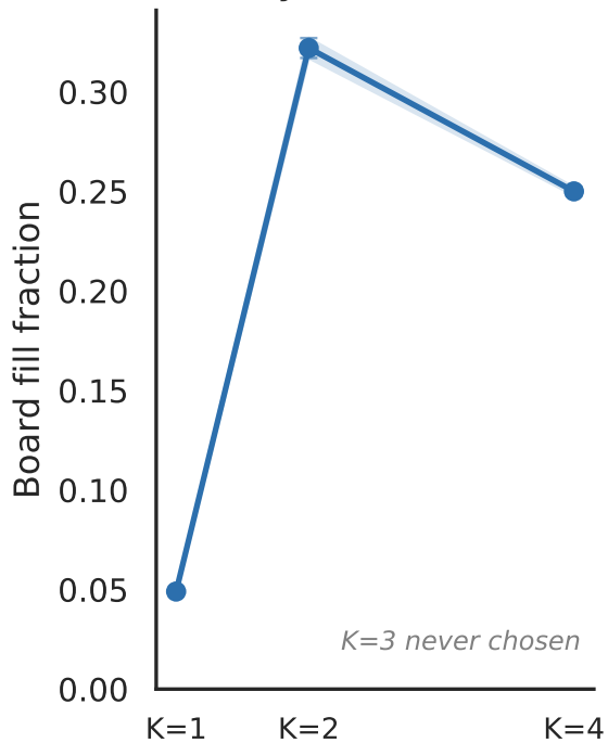
Board density by chosen K
