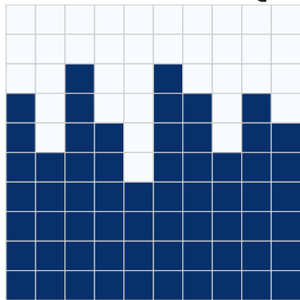
State s_t
