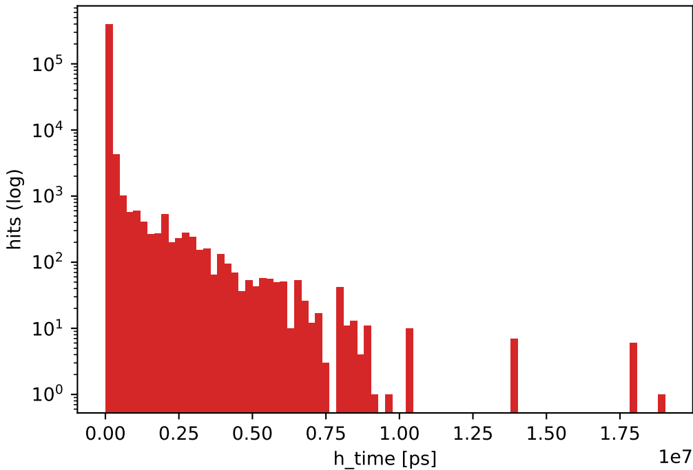
Hit time, full range (late tail = calo backscatter)
