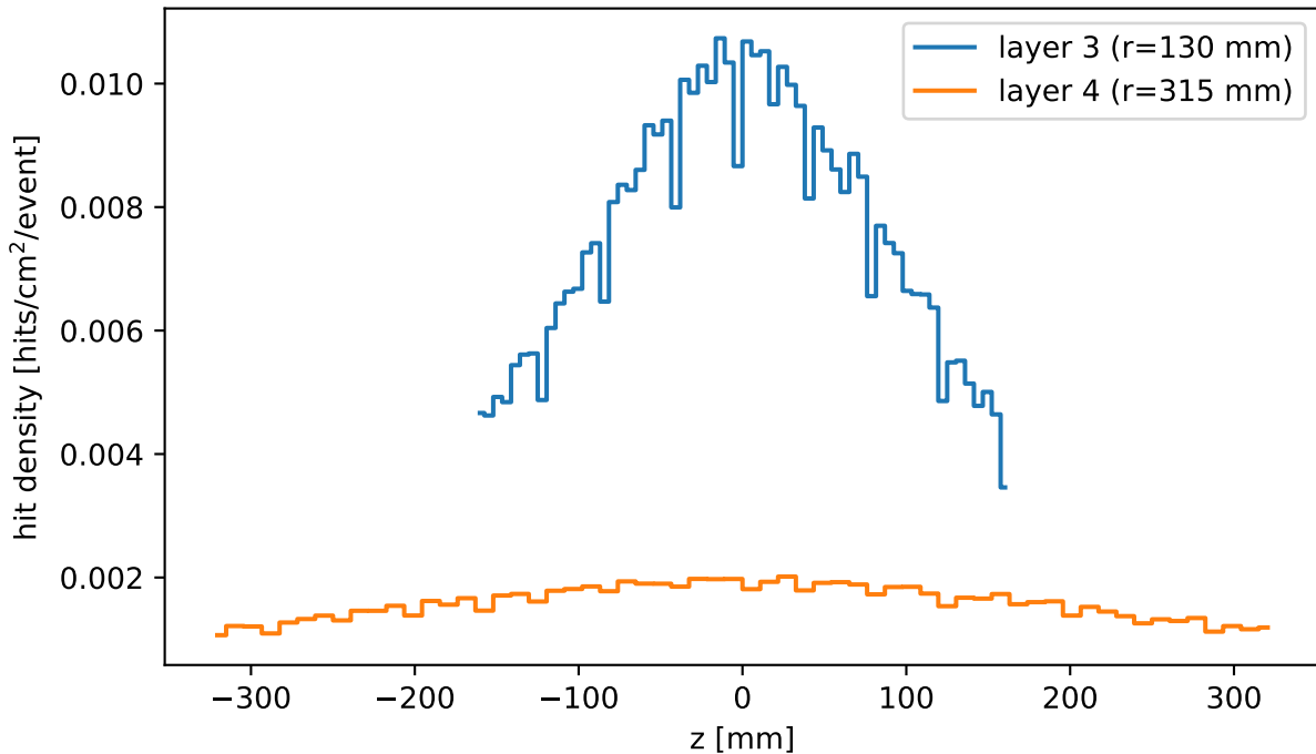
VTXOB occupancy profile vs z (physics only)
