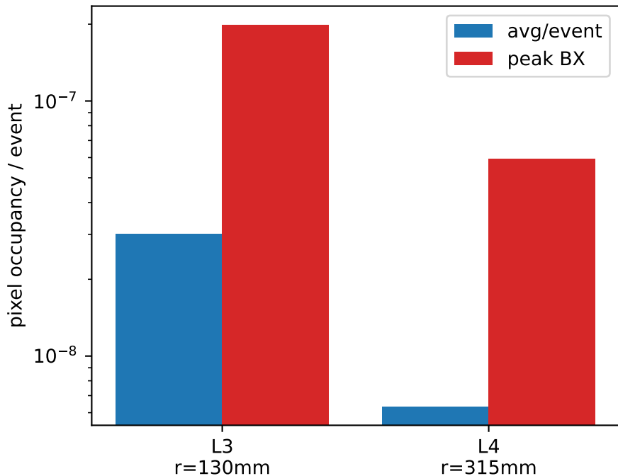
Occupancy per VTXOB layer (20 \mu\text{m} pixels)
