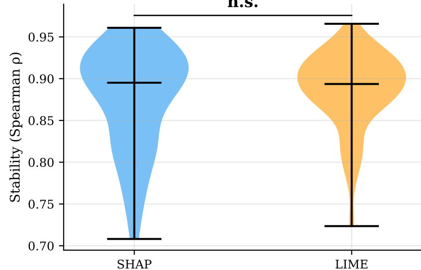
Explanation Stability Under Perturbation n.s.
