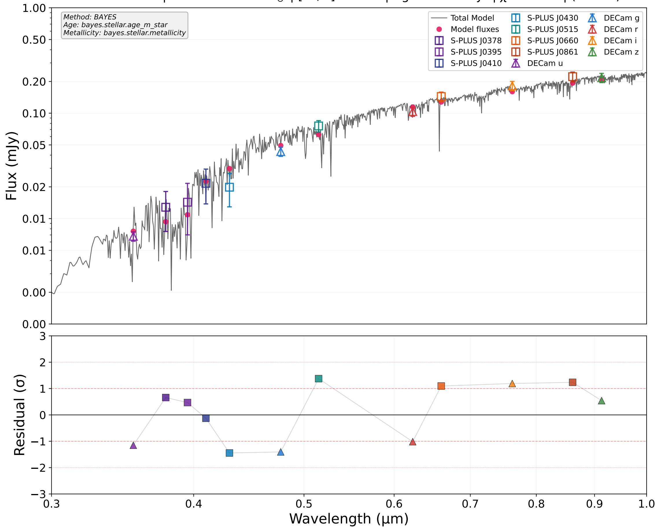
GC T17-2799 | M = 5.51\text{e}+06 M_{\odot} | [\text{Fe}/\text{H}] = 0.30 | Age = 11.4 Gyr | \chi^2 = 1.22 | (BAYES)
