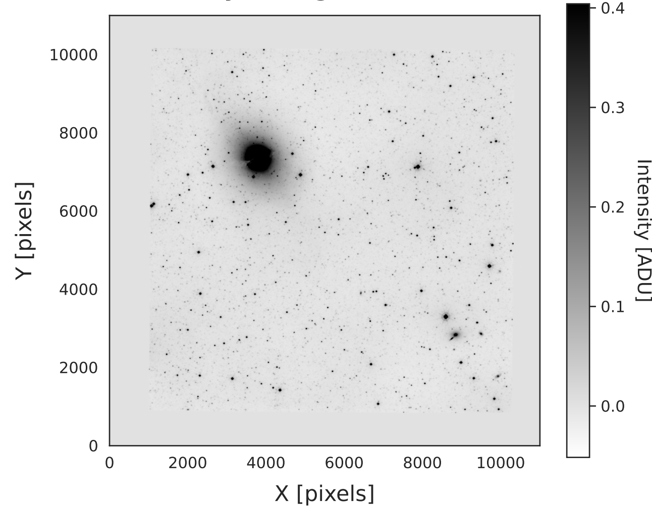
Galaxy Background Model
