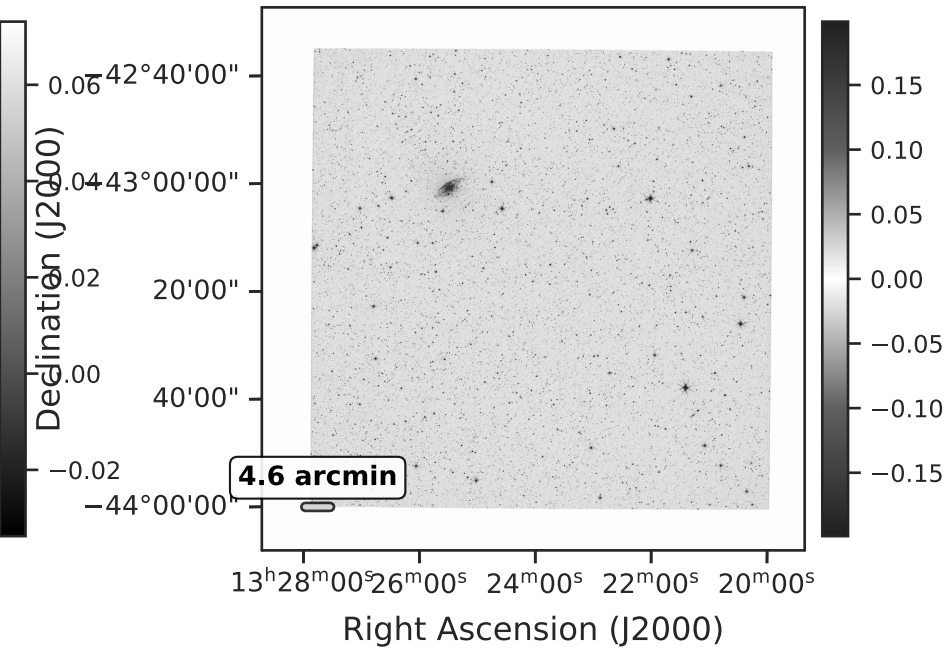
(c) Residual Image
