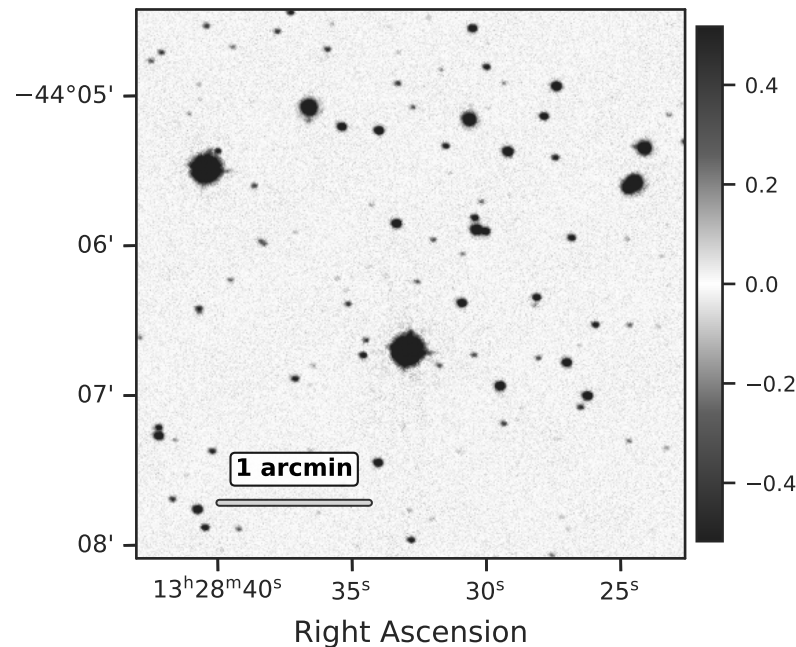
(e) Central Region - Residual
