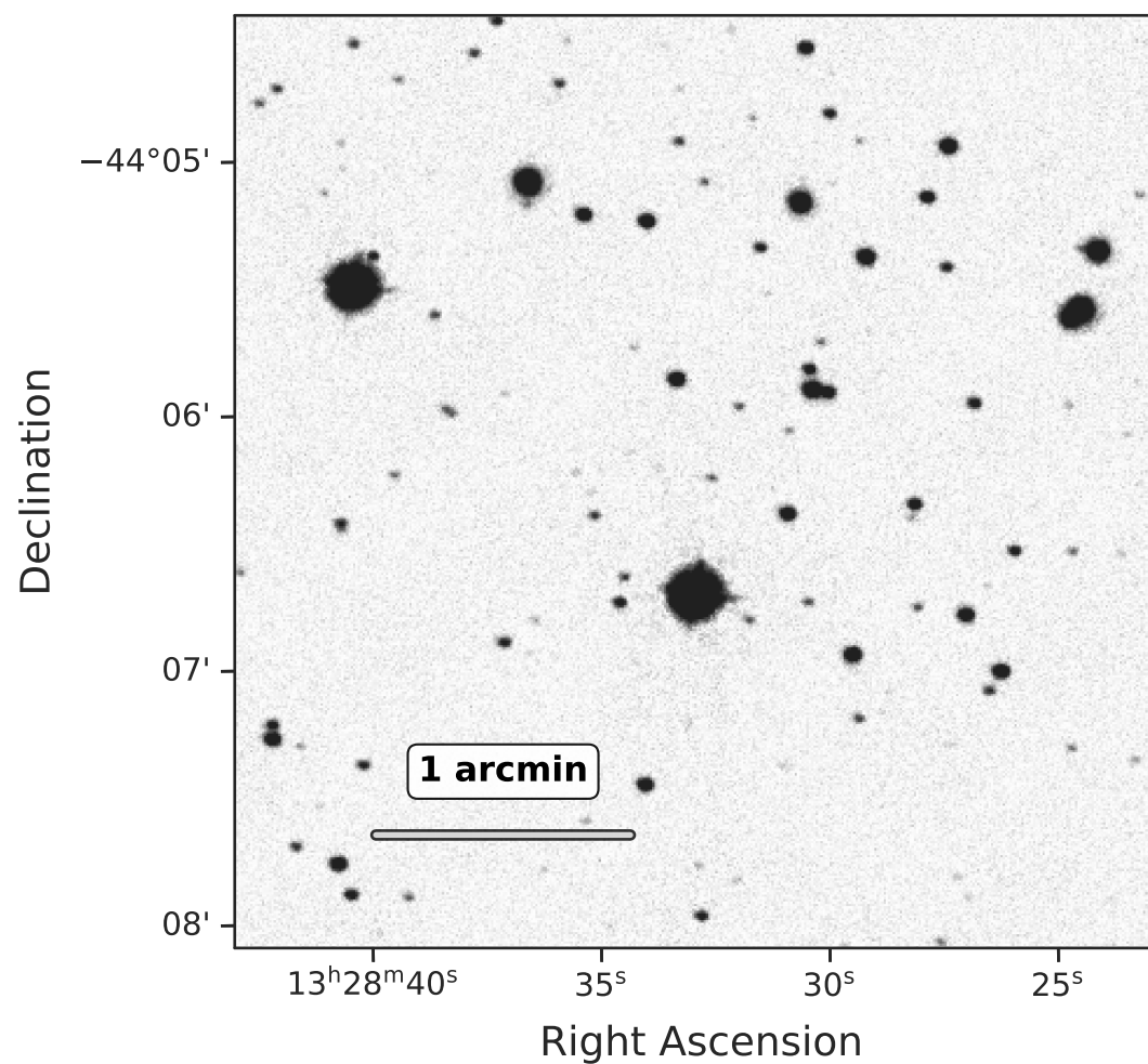
(e) Central Region - Residual
