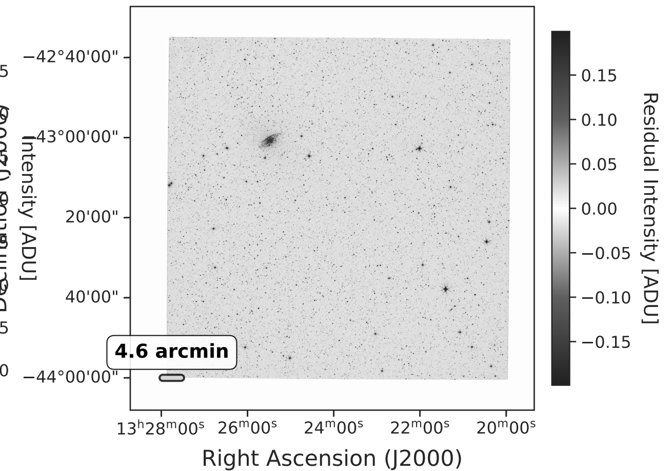
(c) Residual Image
