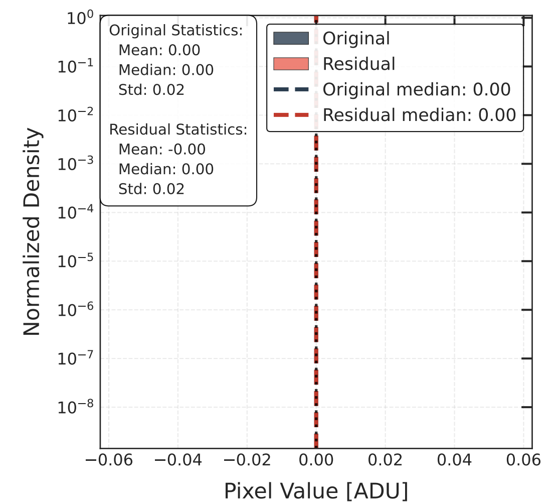
(f) Pixel Value Distribution
