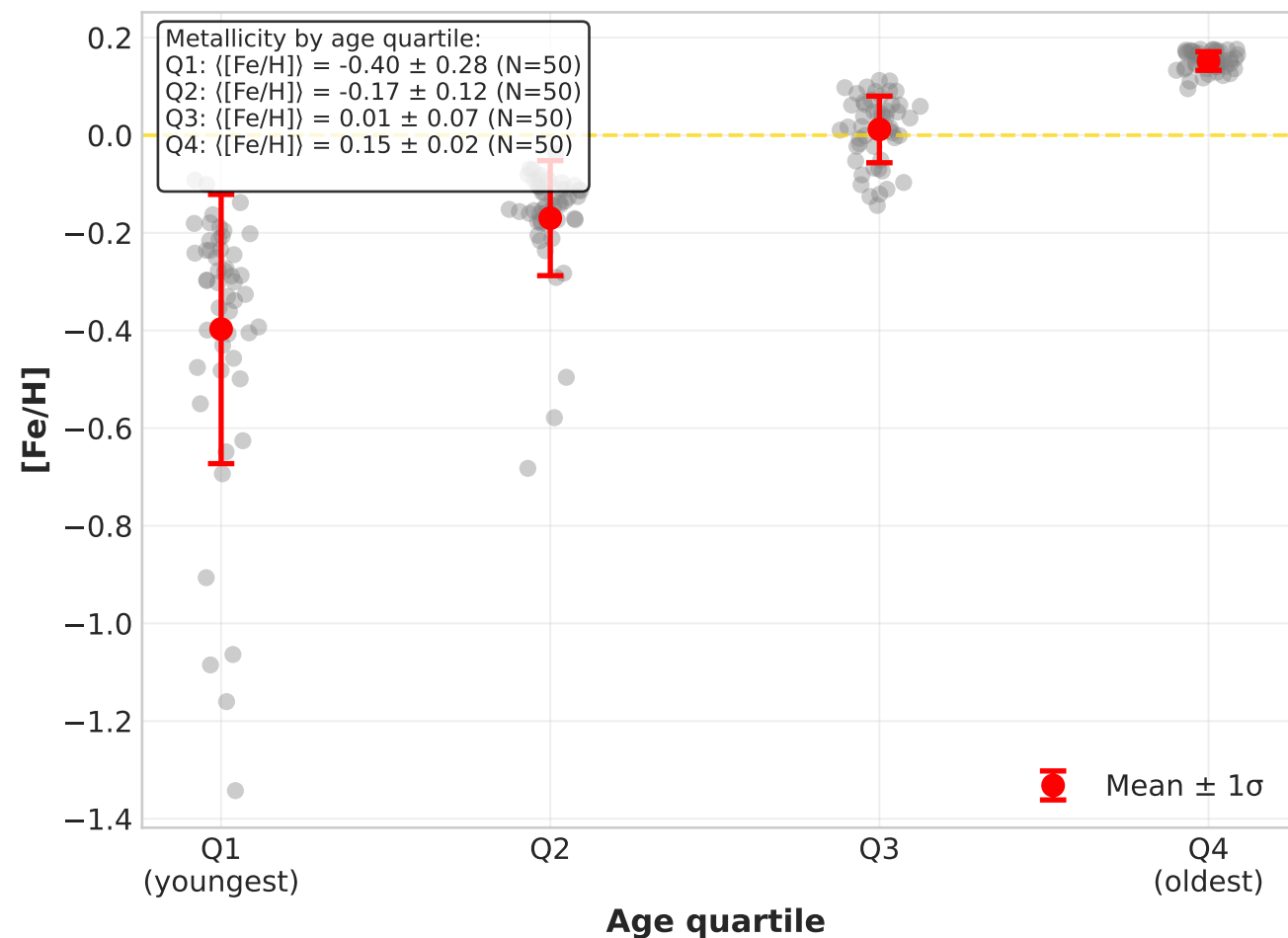
(b) Metallicity by Age Quartile
