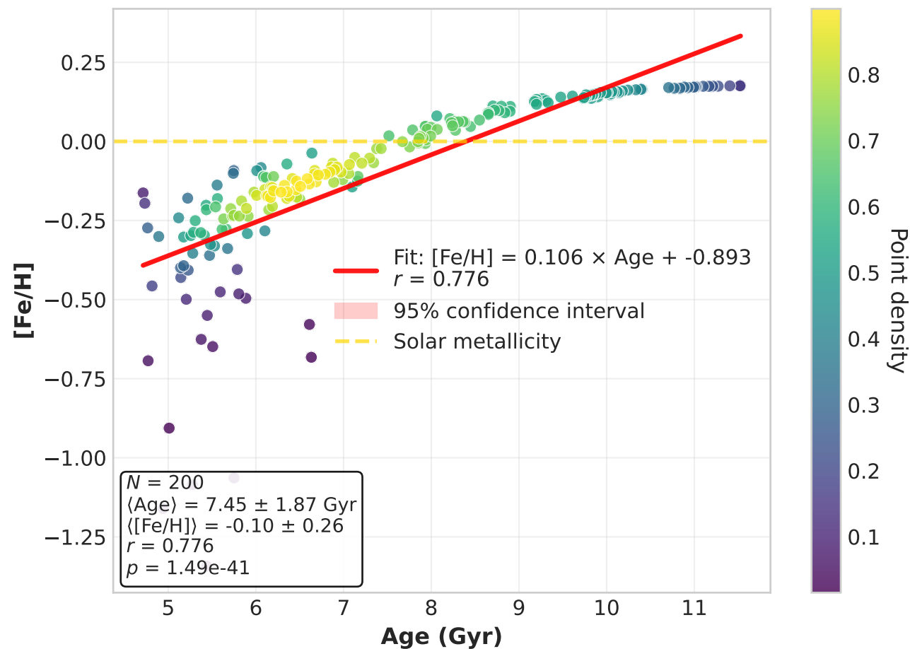
(a) Age-Metallicity Relation
