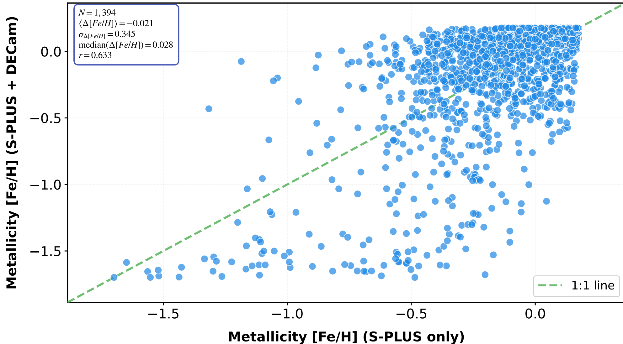
Metallicity Comparison: S-PLUS vs S-PLUS+DECam
