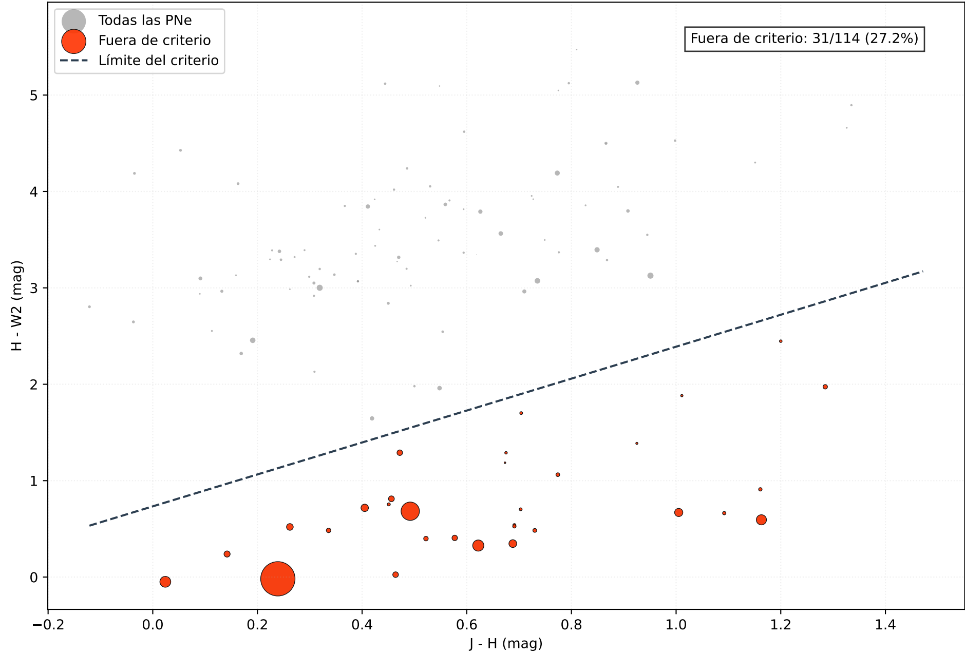
Criterio 3: J-H vs H-W2
