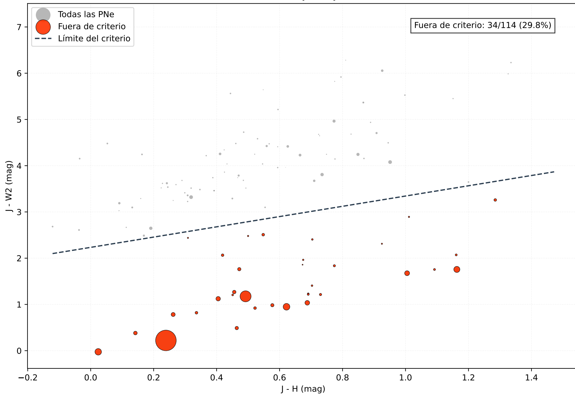
Criterio 5: J-H vs J-W2
