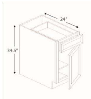
BASE CABINET: 1 Door, 1 Drawer
