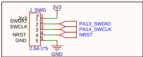
Header SWD (Serial Wire Debug)
