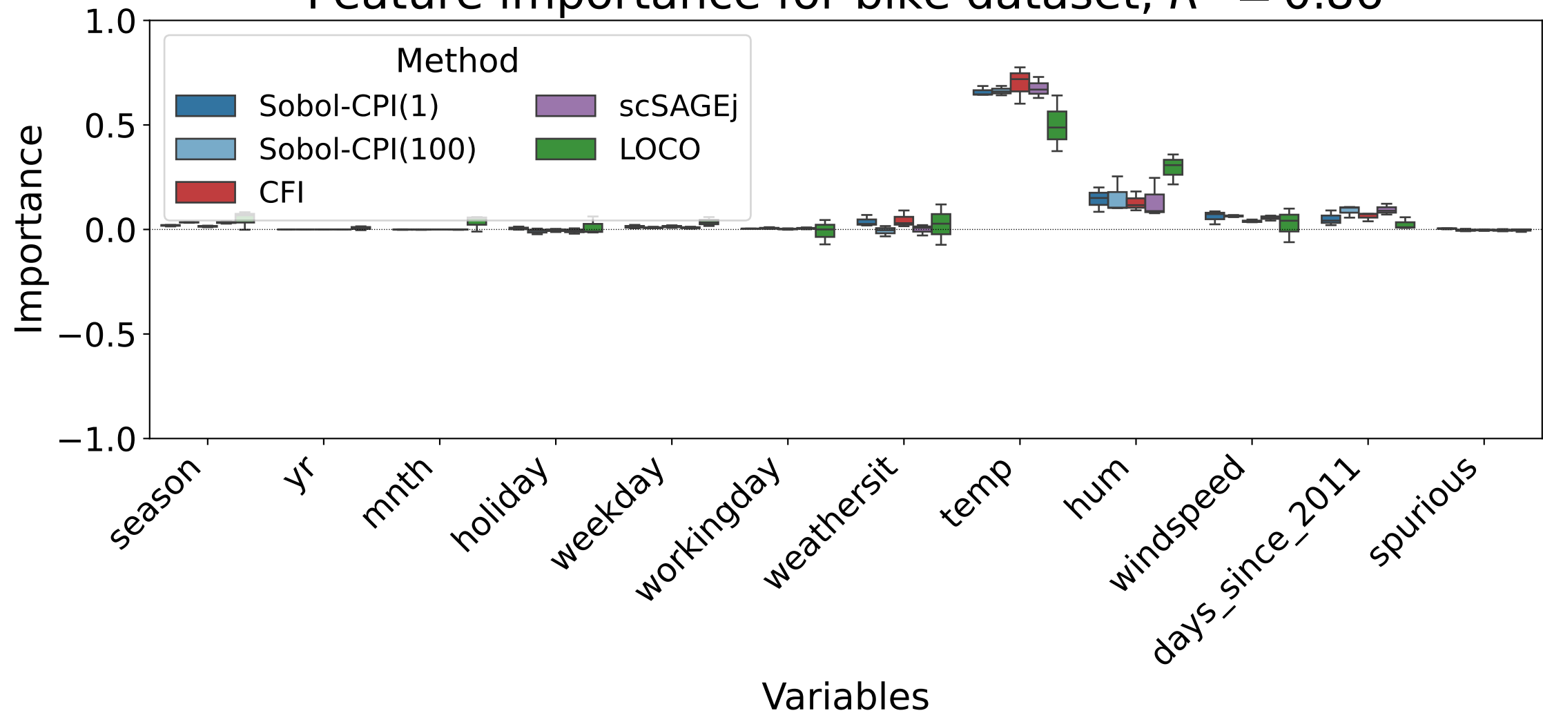
Feature importance for bike dataset, R^2 = 0.86
