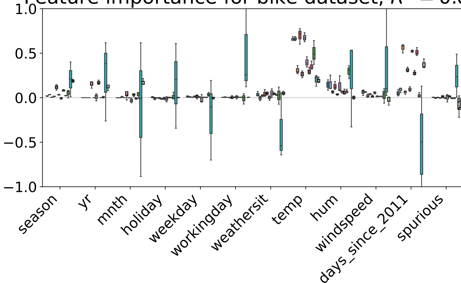
Feature importance for bike dataset, R^2 = 0.86
