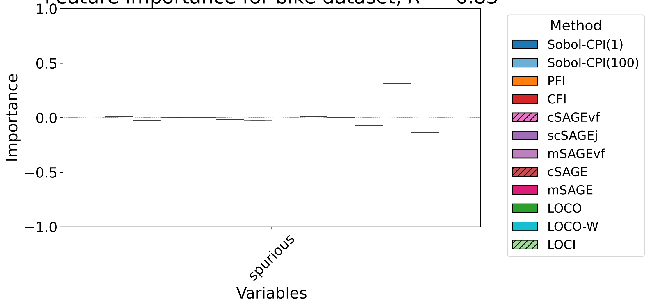
Feature importance for bike dataset, R^2 = 0.83
