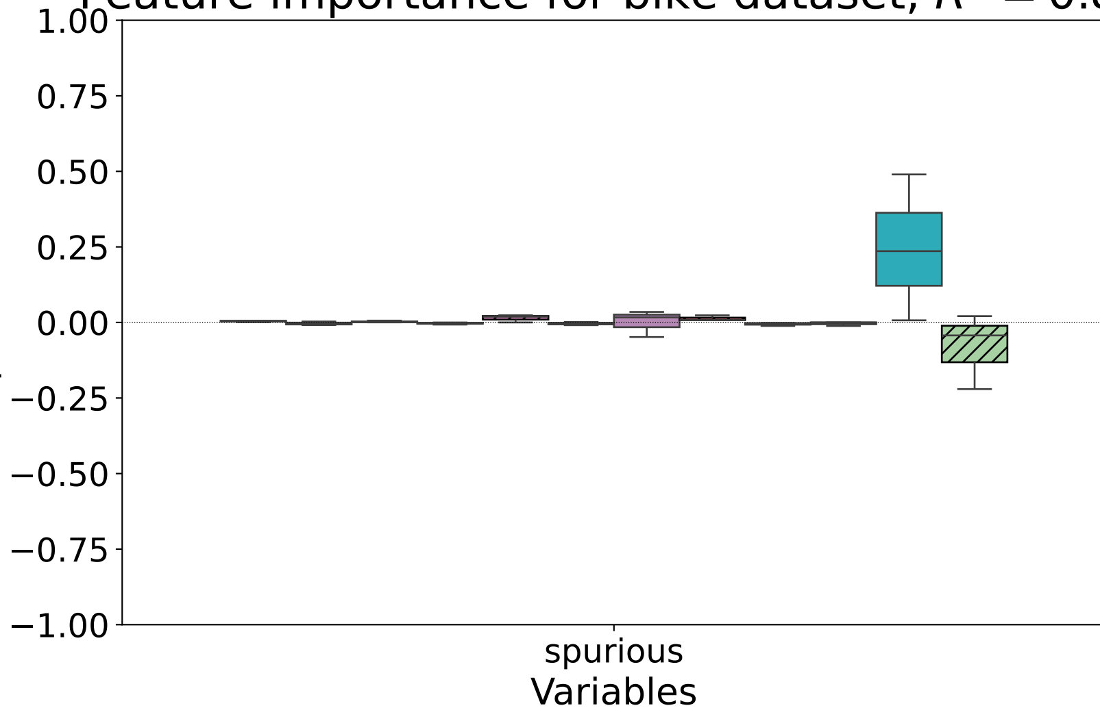
Feature importance for bike dataset, R^2 = 0.86
