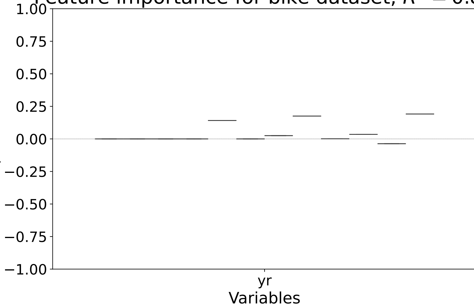
Feature importance for bike dataset, R^2 = 0.88
