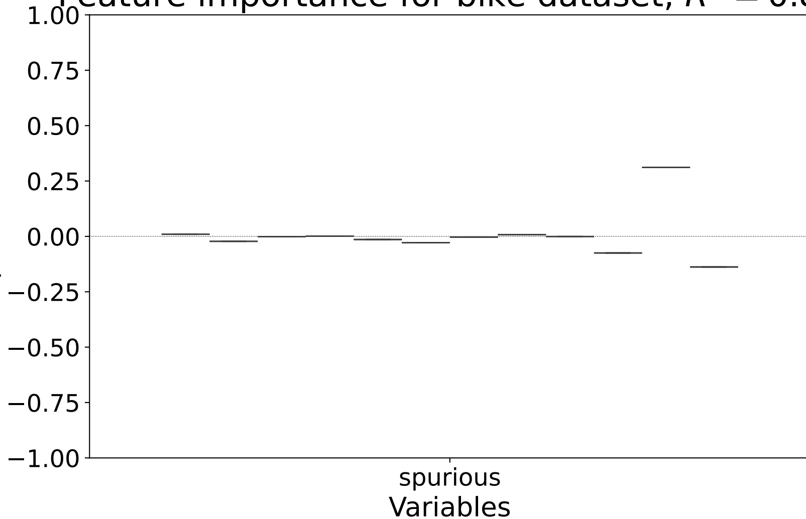
Feature importance for bike dataset, R^2 = 0.83
