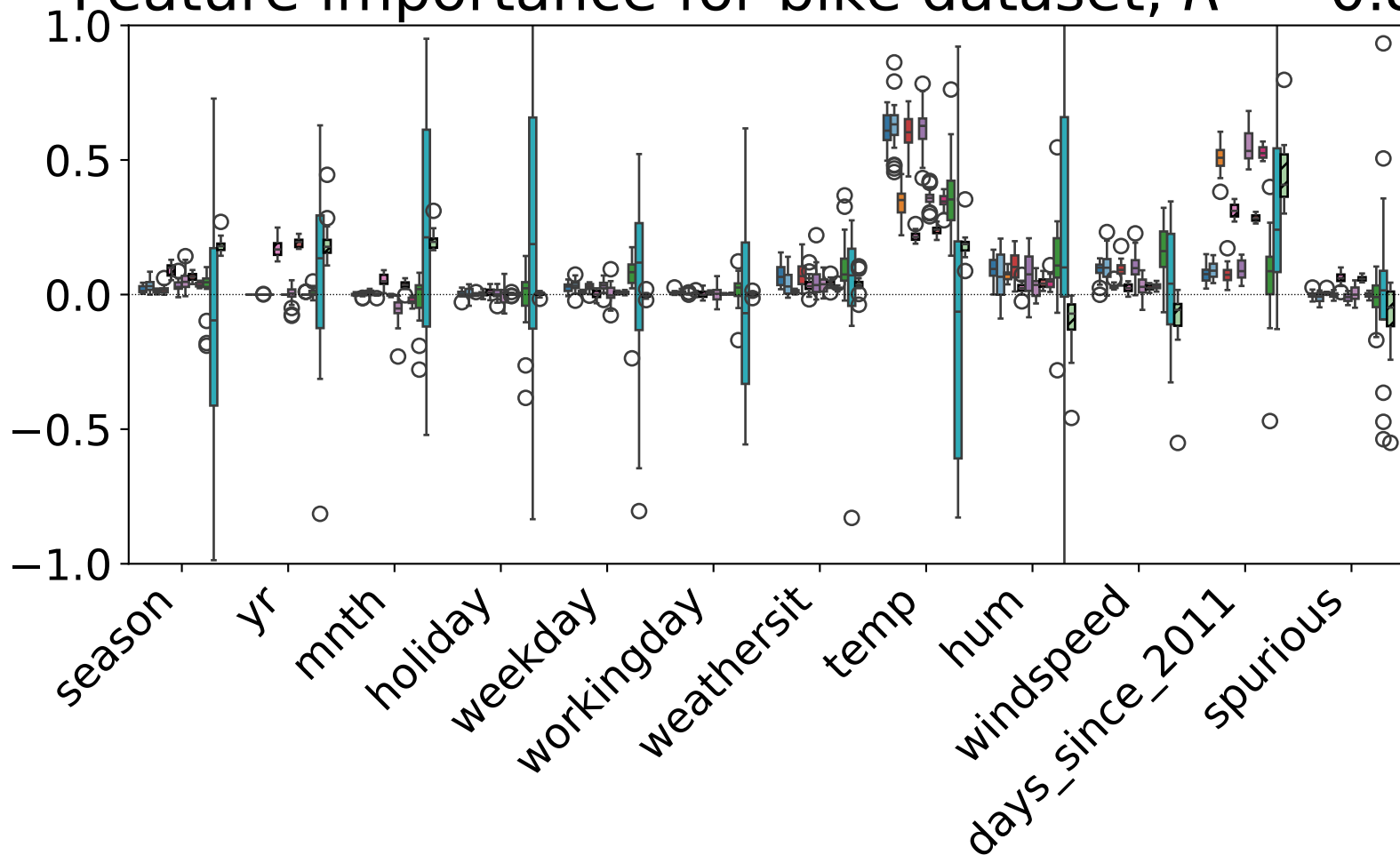
Feature importance for bike dataset, R^2 = 0.89
