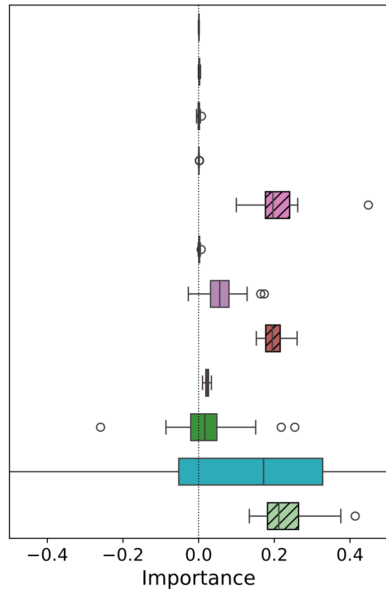
MLP R^2 = 0.79
