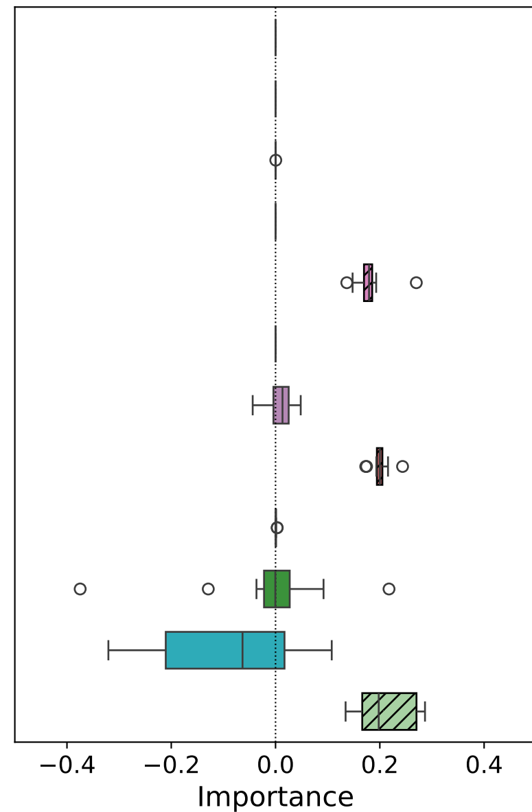
RF R^2 = 0.88
