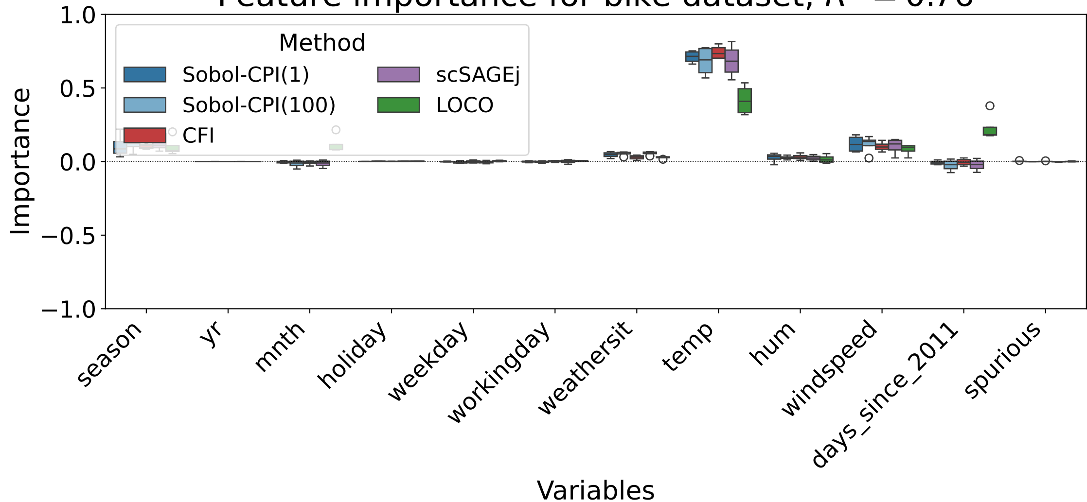
Feature importance for bike dataset, R^2 = 0.76
