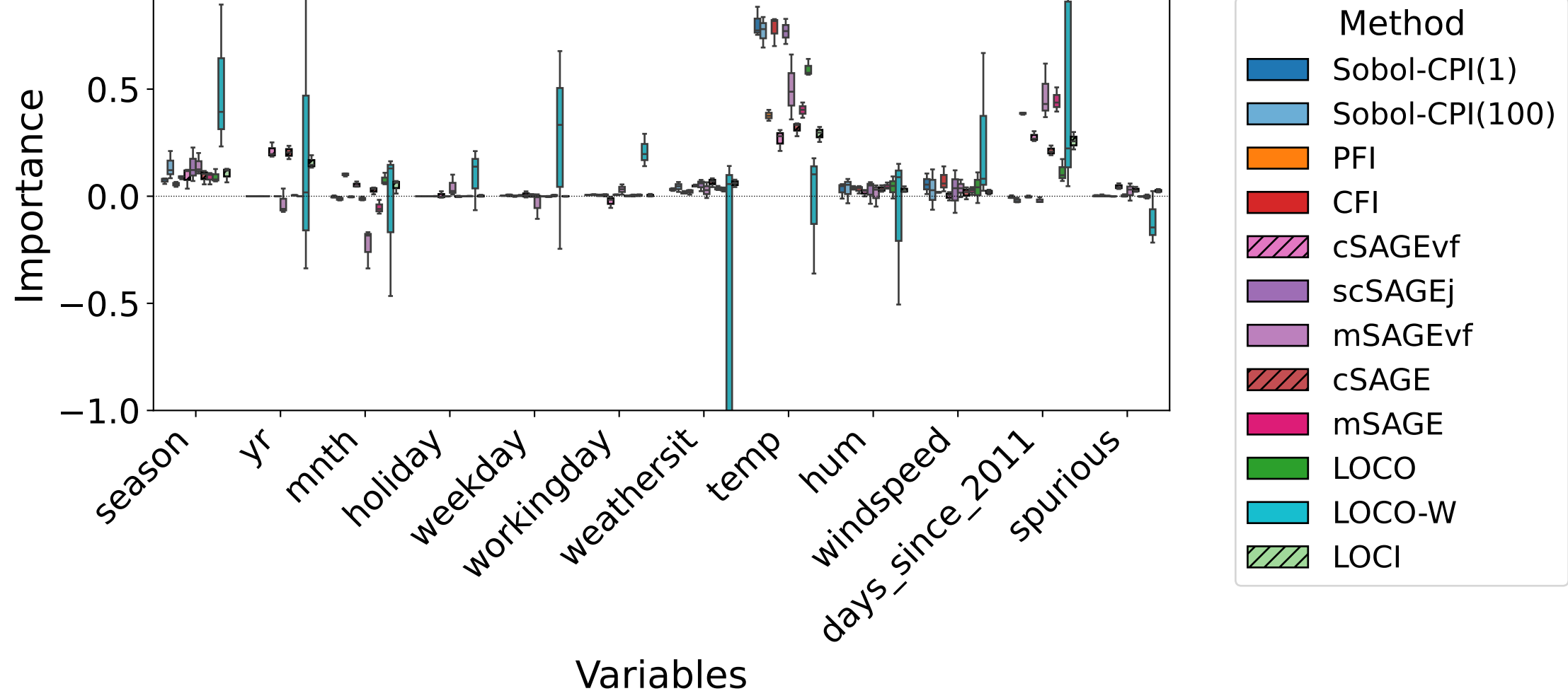
Feature importance for bike dataset, R^2 = 0.72
