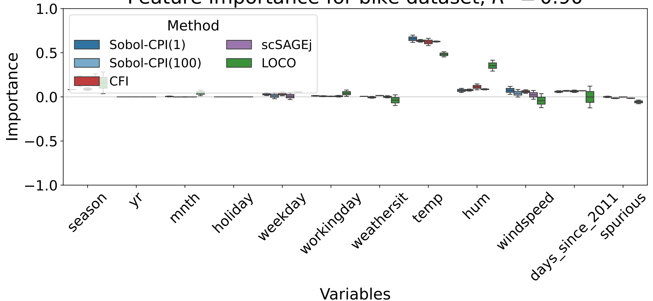
Feature importance for bike dataset, R^2 = 0.90
