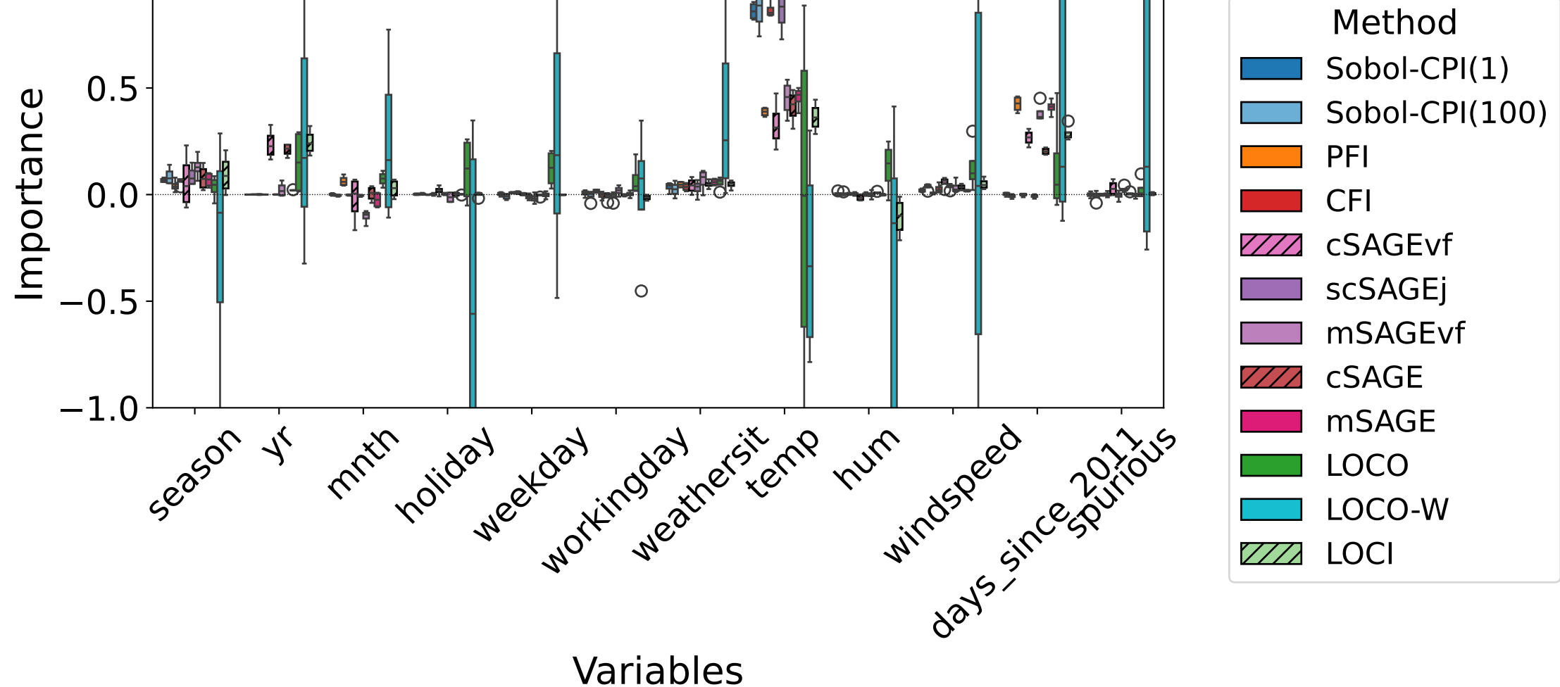
Feature importance for bike dataset, R^2 = 0.74
