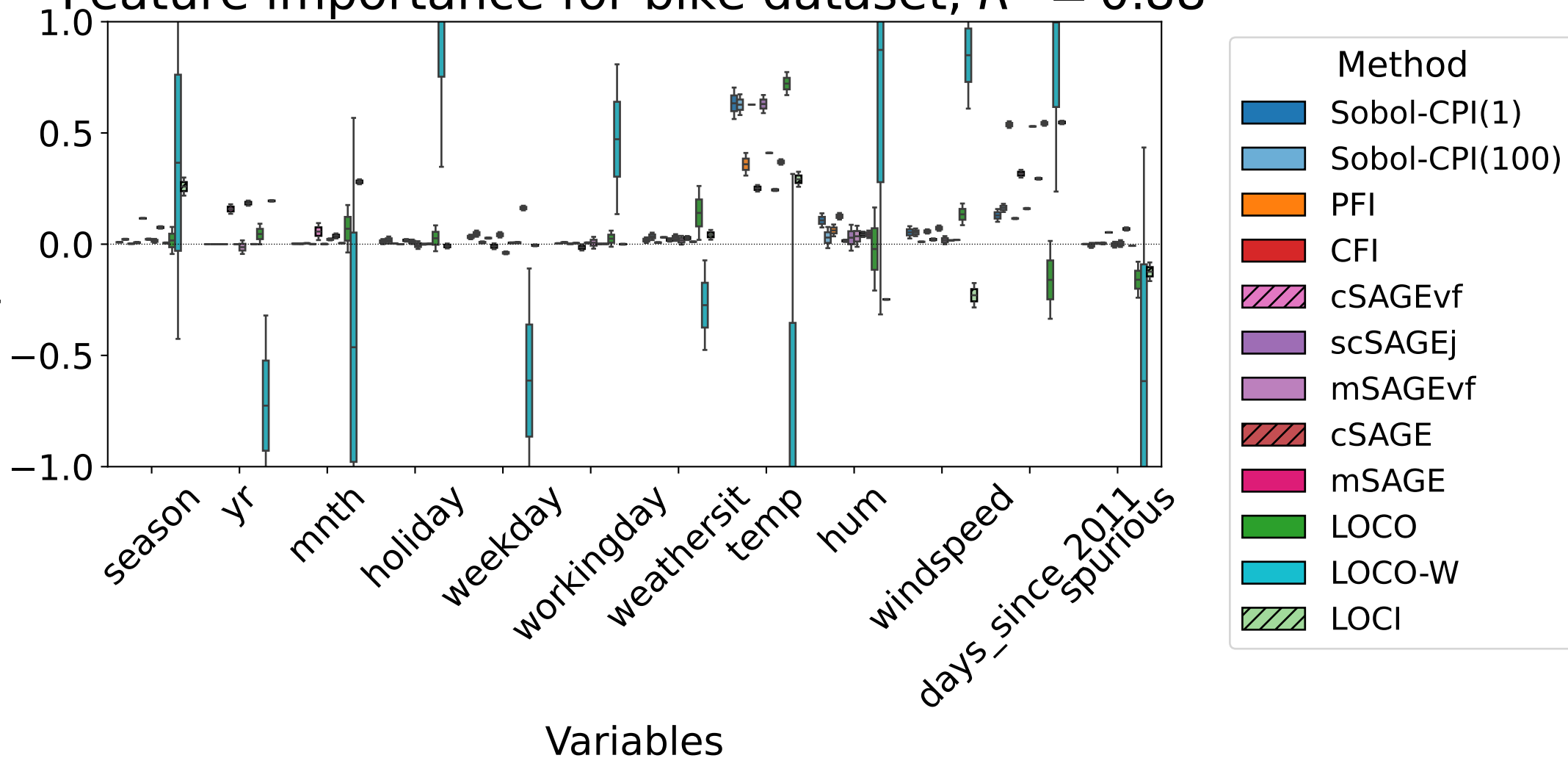
Feature importance for bike dataset, R^2 = 0.88
