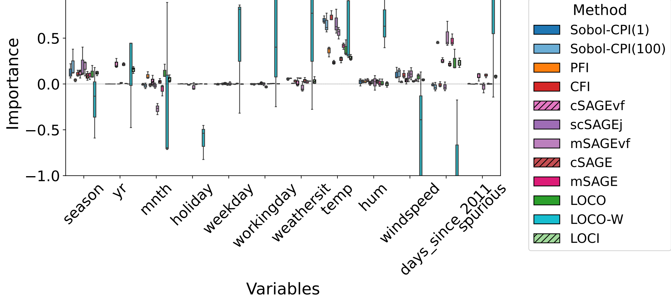
Feature importance for bike dataset, R^2 = 0.76
