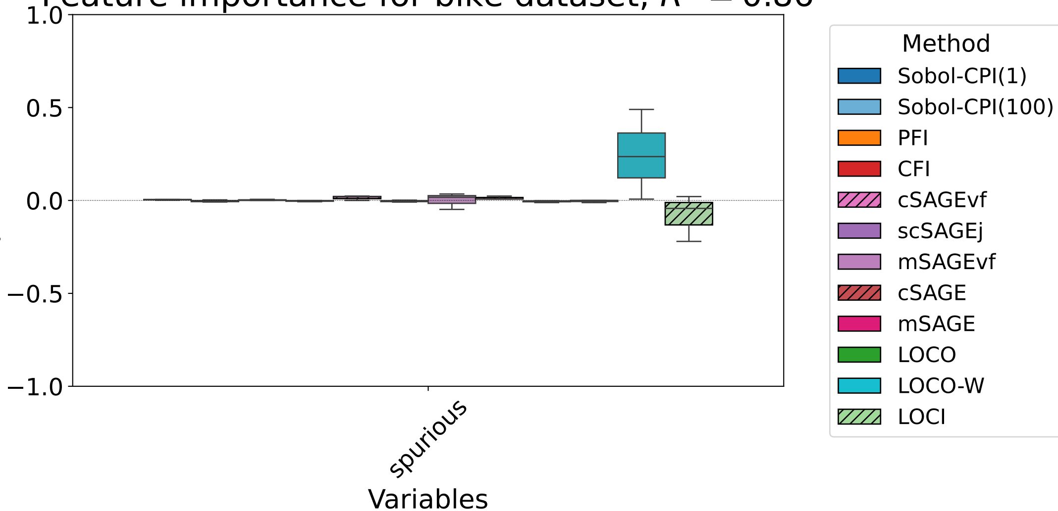
Feature importance for bike dataset, R^2 = 0.86
