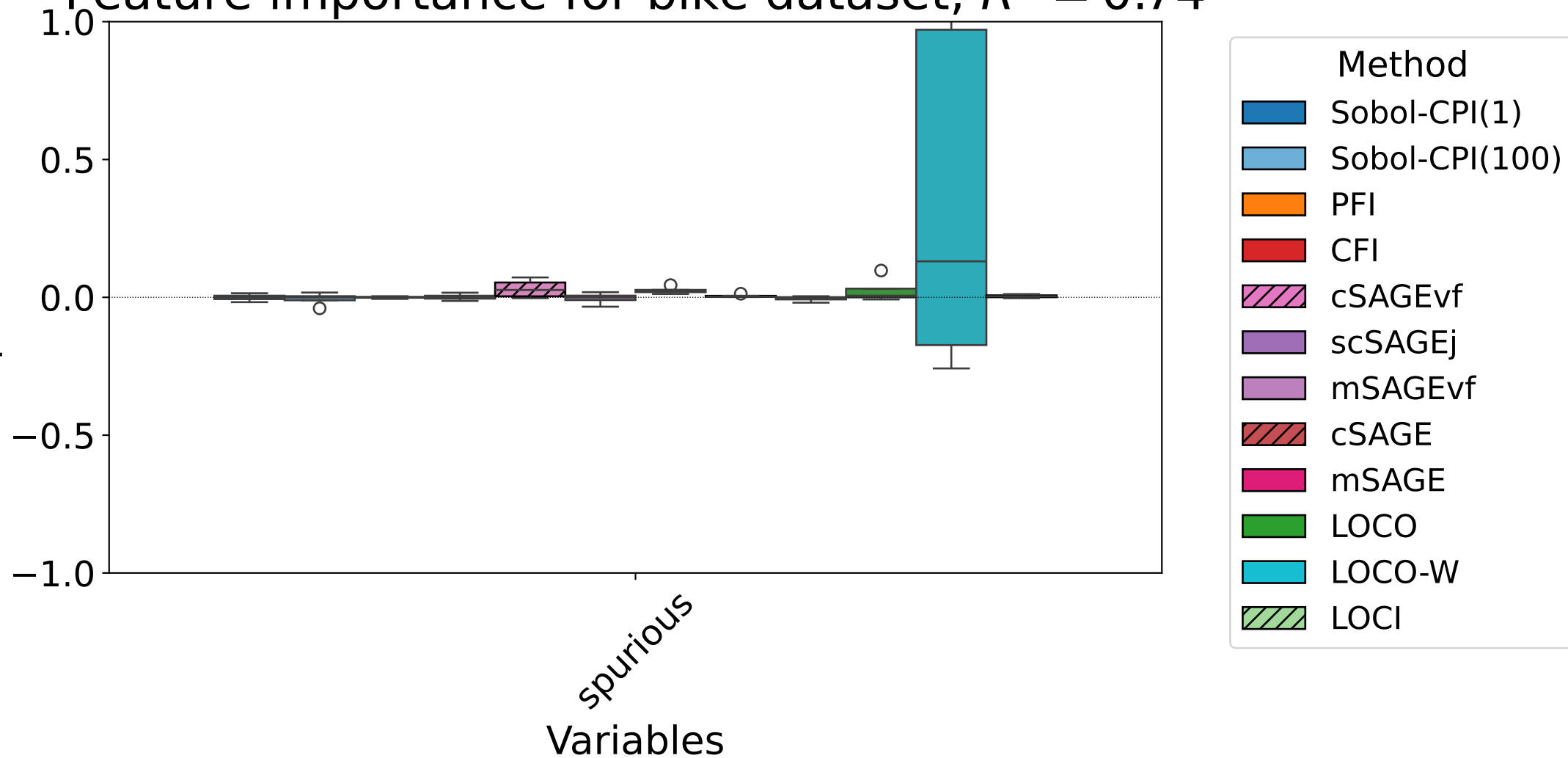
Feature importance for bike dataset, R^2 = 0.74
