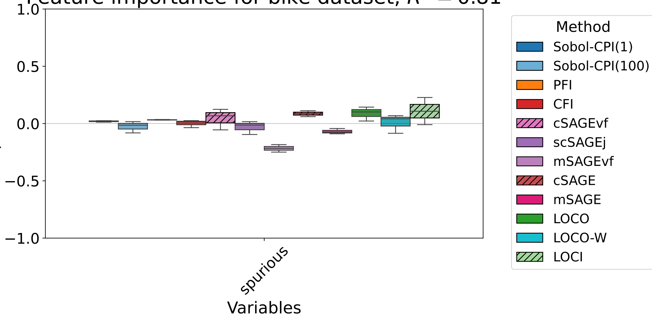
Feature importance for bike dataset, R^2 = 0.81
