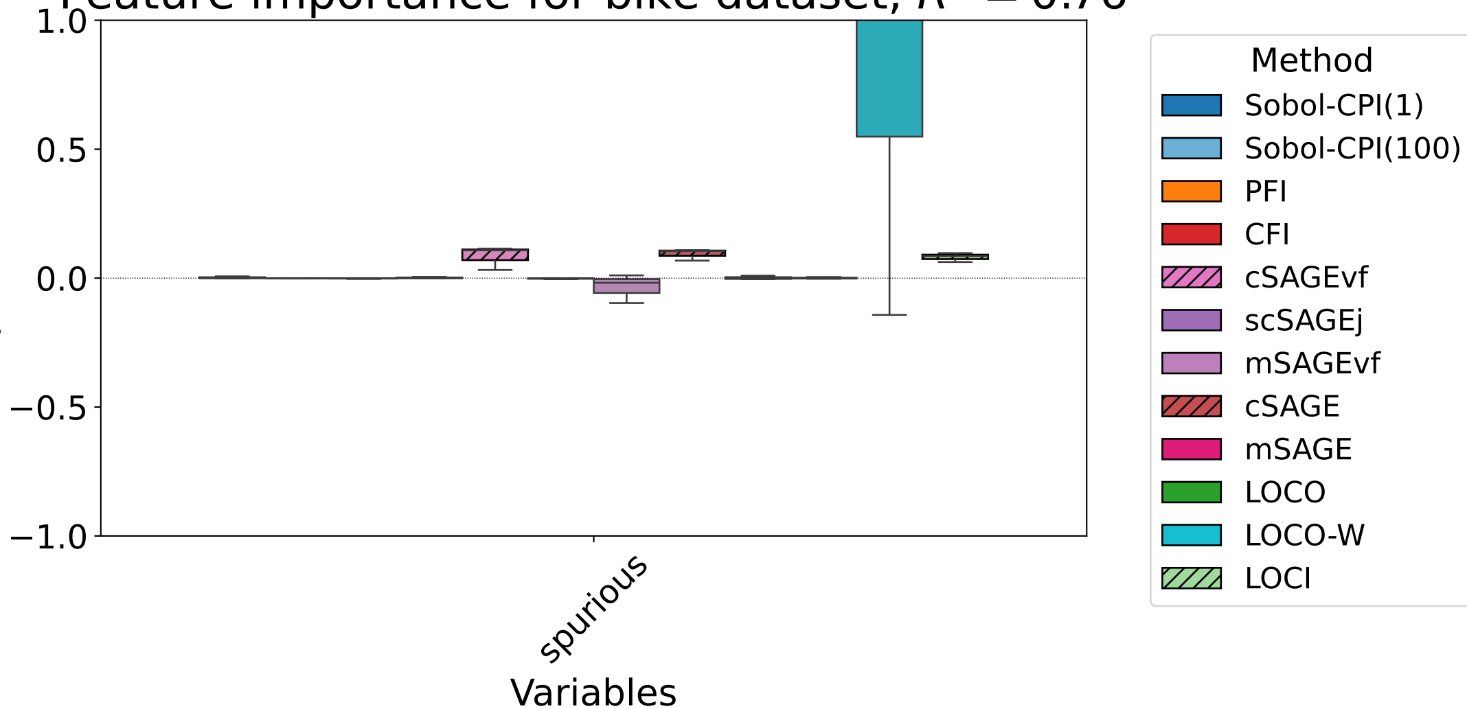
Feature importance for bike dataset, R^2 = 0.76
