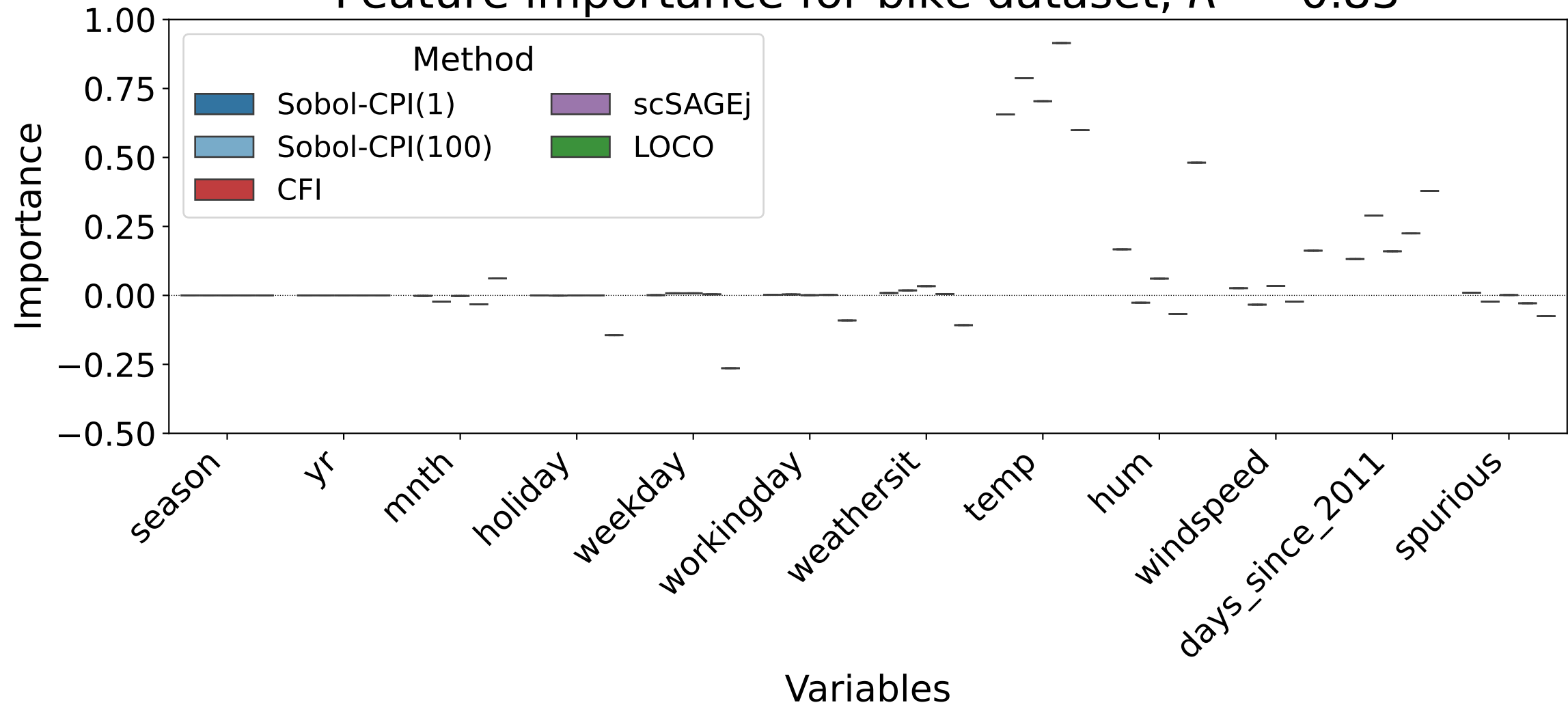
Feature importance for bike dataset, R^2 = 0.83
