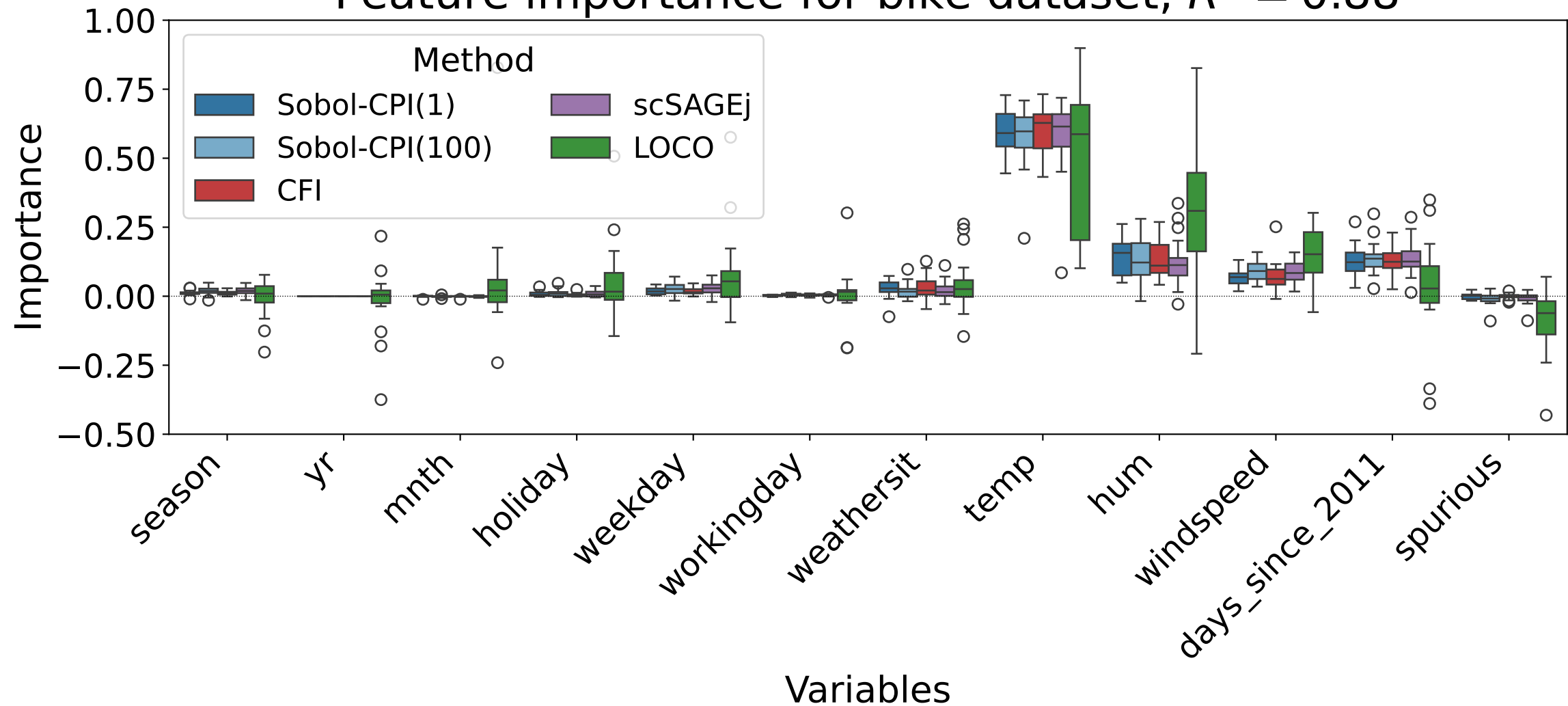
Feature importance for bike dataset, R^2 = 0.88
