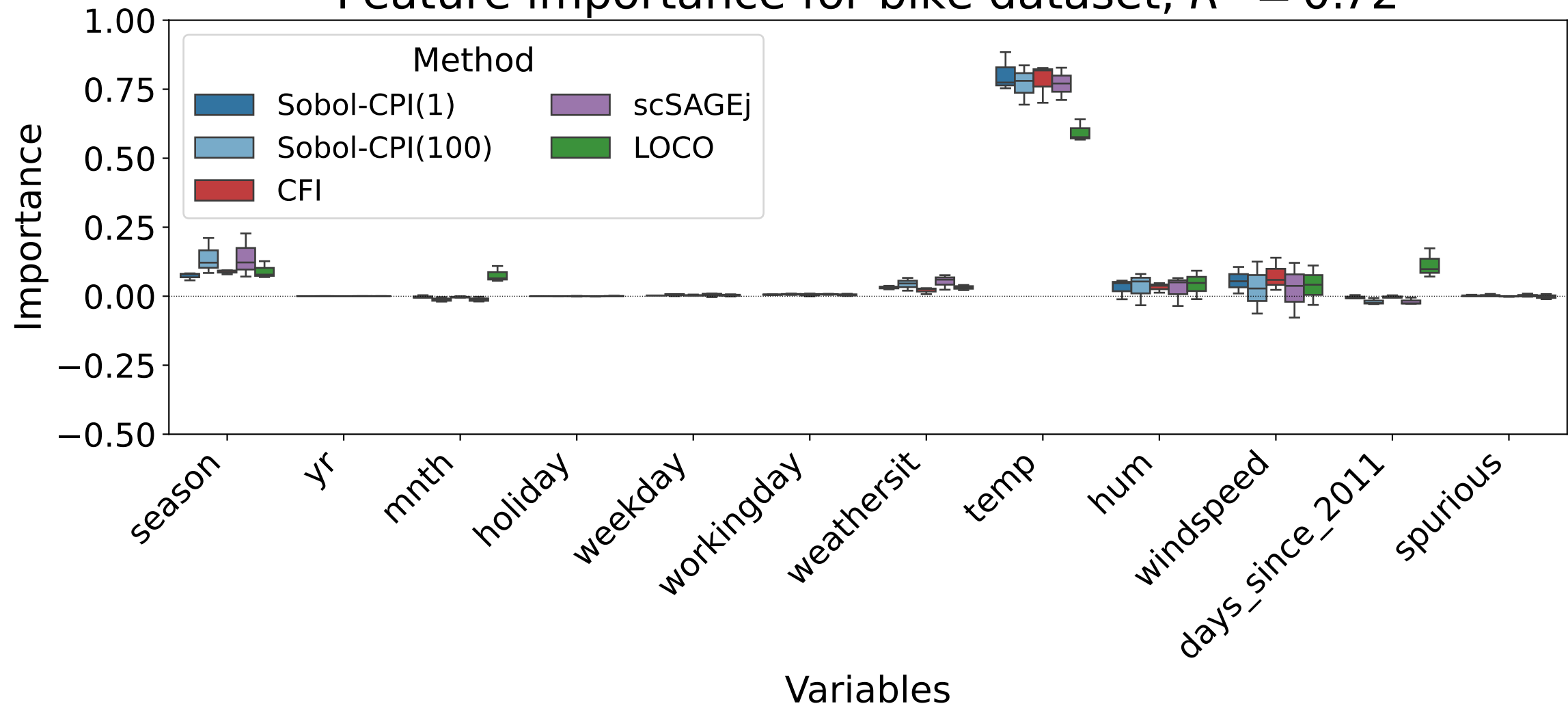
Feature importance for bike dataset, R^2 = 0.72
