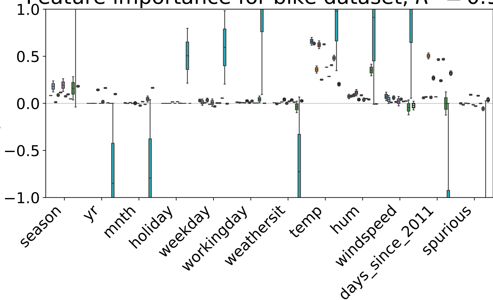
Feature importance for bike dataset, R^2 = 0.90
