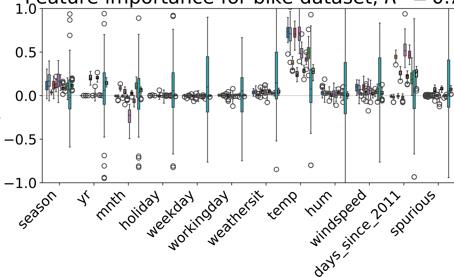
Feature importance for bike dataset, R^2 = 0.76
